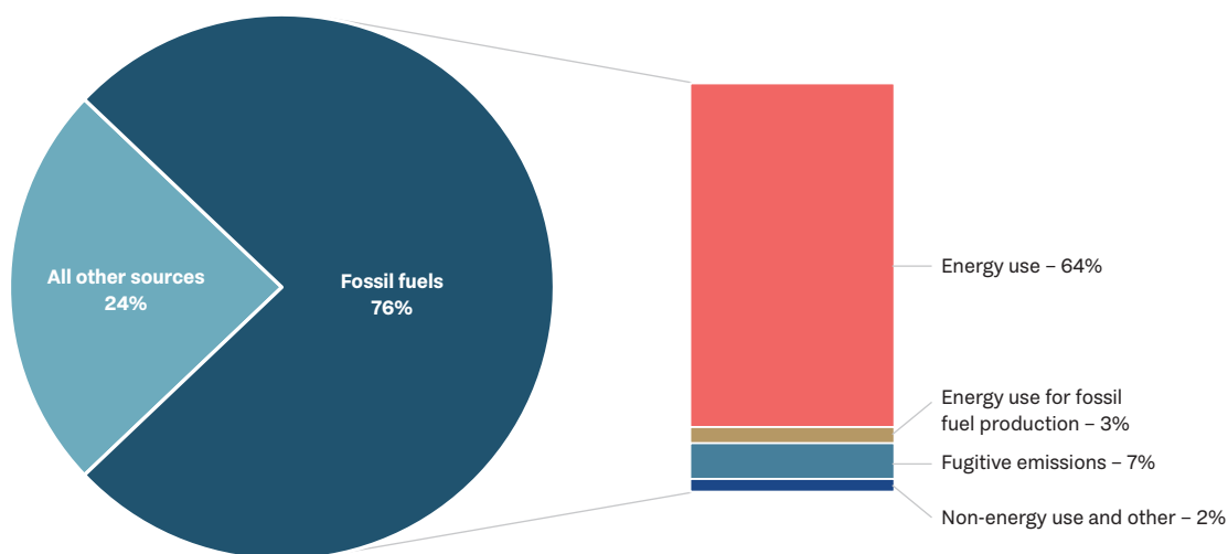
Global greenhouse gas emissions by source
